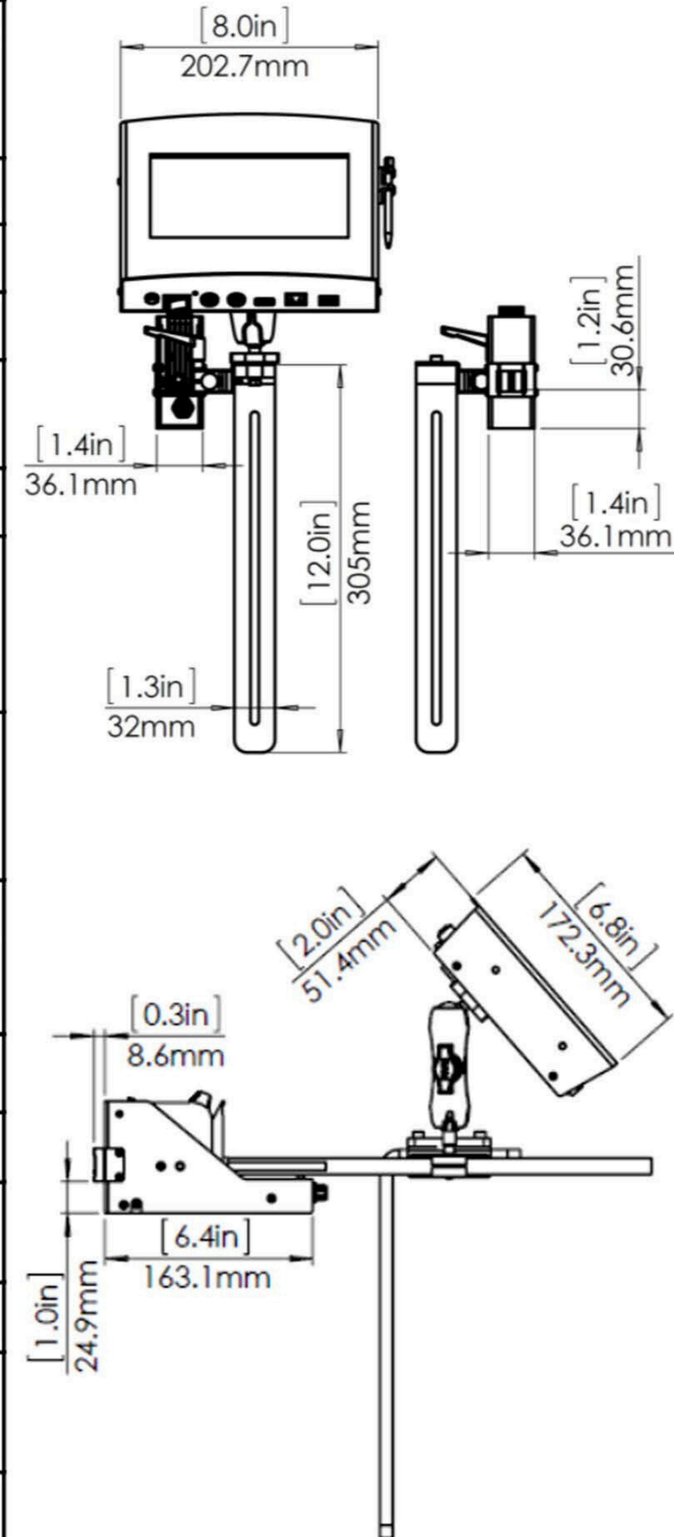
Dimensions are in mm [inch]
